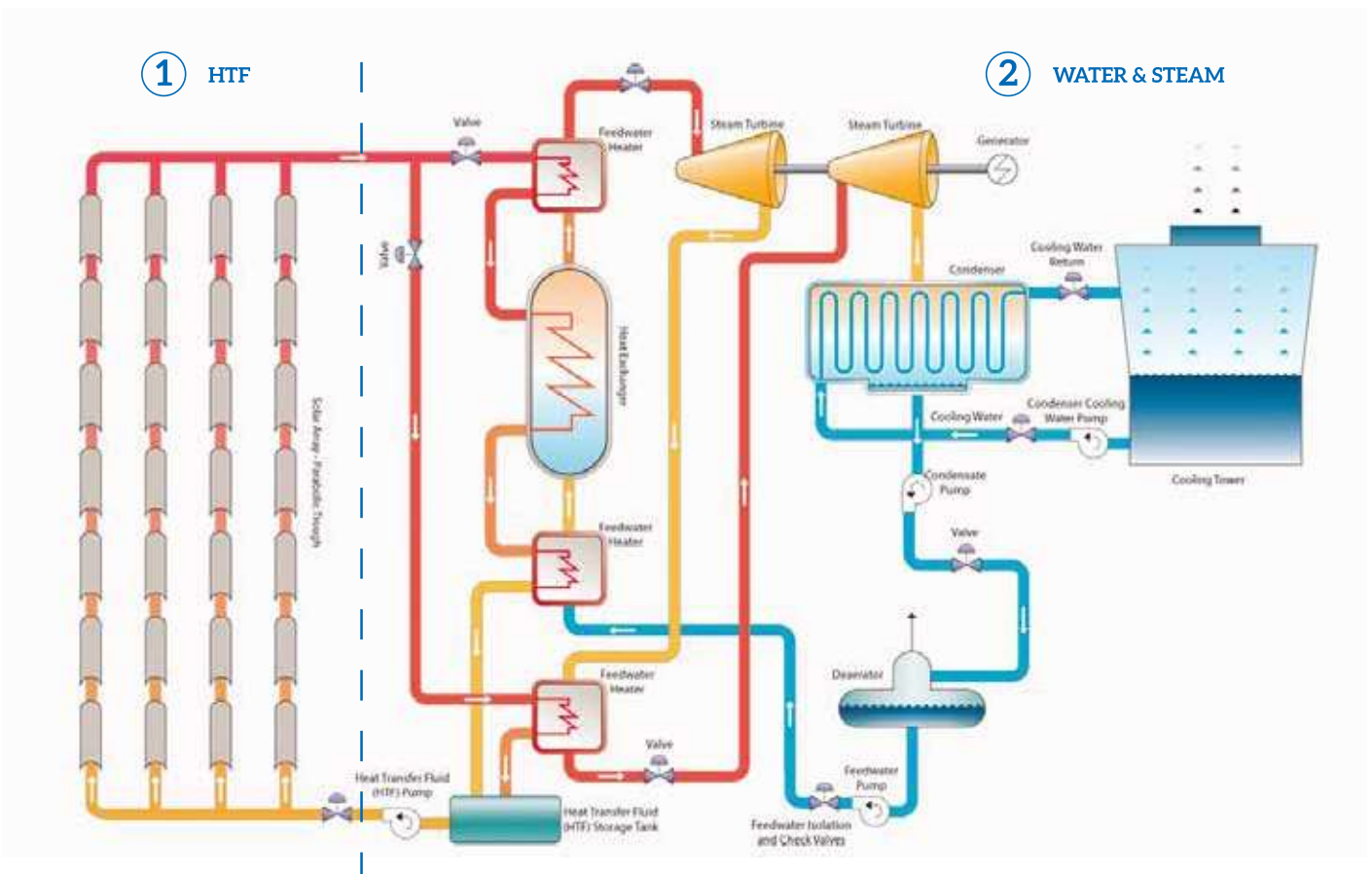
Diagram of a Parabolic Trough CSP without molten salts storage
